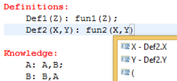
Figure 5. Local variables’ UI consequences
