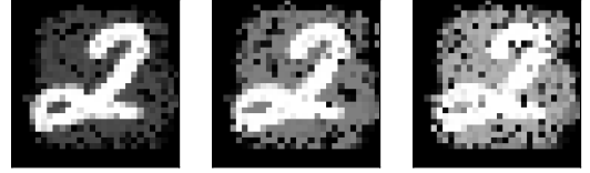
Figure 5: Instances generated by Z3 for \epsilon \in \{0.3, 0.5, 0.7\} .
