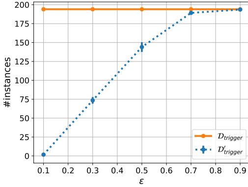
Figure 4: Size of the forged trigger set D'_{\text{trigger}} when varying the amount of distortion \epsilon on the MNIST2-6 dataset.
